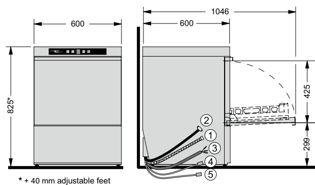
Undercounter dishwasher model F515
