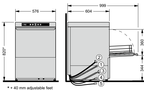
Undercounter dishwasher model F504
