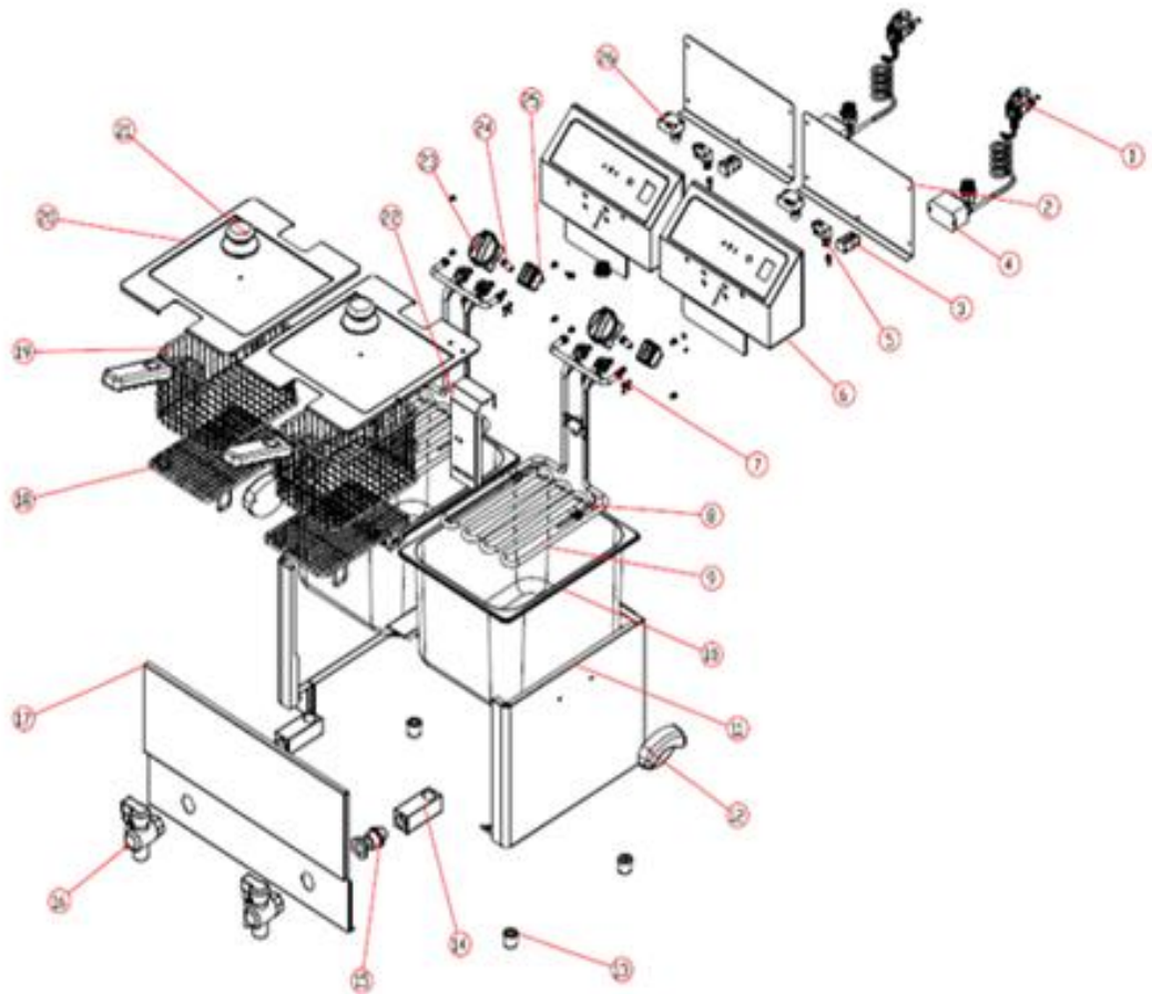
HDF Series 1-tank electric fryer
