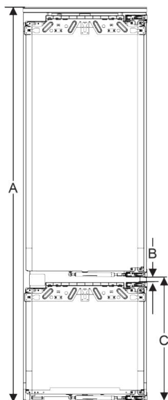
Fig. 68 Clearances for a 2-door
